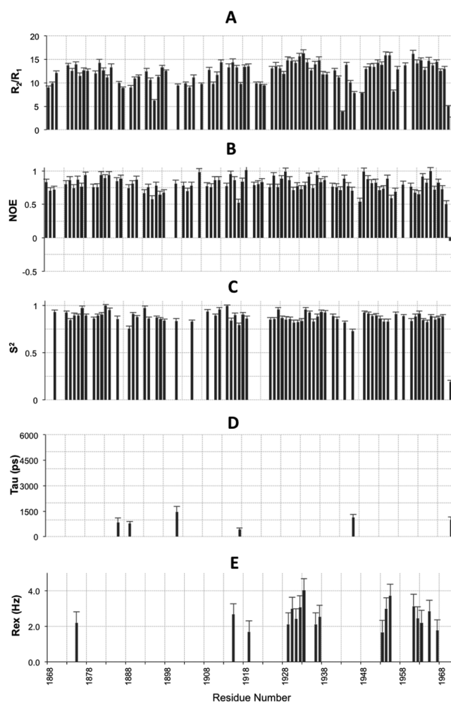
Figure 3. Parameters describing internal dynamics for the assigned and nonoverlapping residues of BAZ2B bromodomain. (A) ^{15}\text{N} -R2/R1 ratios; (B) ^{15}\text{N}\{^1\text{H}\} -heteronuclear NOE values; (C) squared general order parameters, S^2 ; (D) fast (ns–ps) internal motions expressed as internal correlation times, \tau_i (ps); (E) slow (ms– \mu s) dynamics expressed as exchange contribution to the line shape, R_{ex} (Hz).
