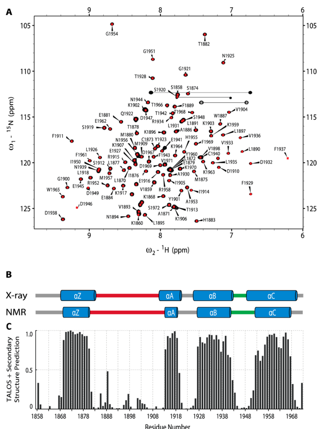
Figure 2. BAZ2B spectral assignment (A) 2D [ ^{15}\text{N} - ^1\text{H} ]-HSQC showing the assignment of BAZ2B bromodomain backbone amide peaks. (B) Comparison of the NMR secondary structure prediction to that seen in the X-ray structure of this construct (PDB ID 3G0L). (C) Secondary structure prediction using Talos+ (bars represent \alpha helix propensity).
