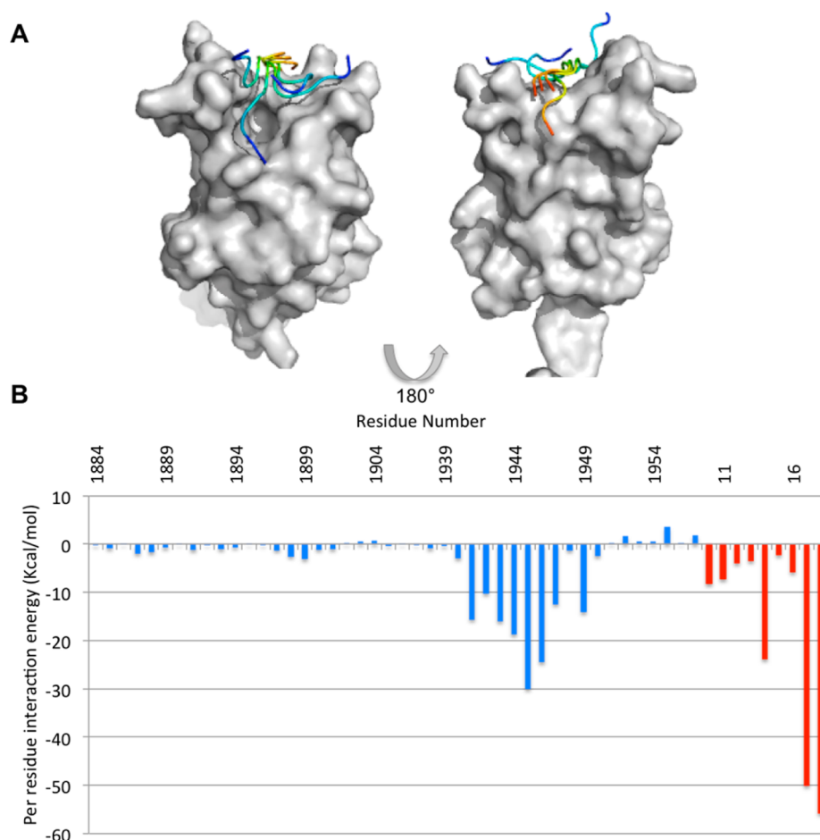
Figure 8. Results of HADDOCK docking (A) Overlay of the top scored models from the top four clusters. (B) Per residue interaction energy (sum of van der Waals and electrostatic energies) for interacting residues in the protein (blue) and peptide (red). Values are shown as an average over the ensemble of output HADDOCK poses.
