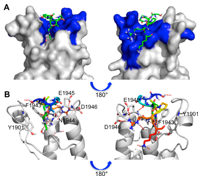
Figure 9. (A) Surface view of the HADDOCK model of the BAZ2B/Peptide 1 complex in closest agreement with experimental data. Residues with CSPs upon titration of Peptide 1 are colored blue. (B) Alternate view of the HADDOCK model, BAZ2B shown gray, interacting residues shown as sticks, H-bonds shown as red dashed lines.
